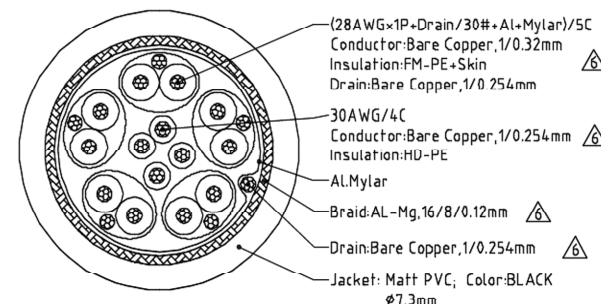
Wire Details
