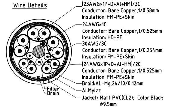
Wire Details
