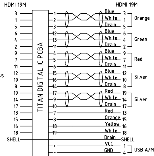
PIN ASSIGNMENT
