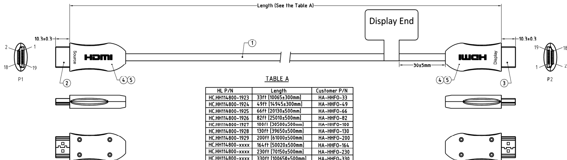
Wire Details
