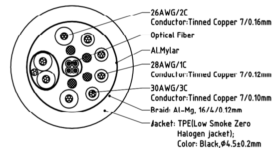
Wire Details
