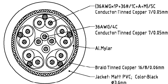
Wire Details
