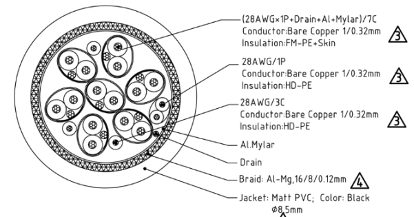
Wire Details(Scale 8:1)
