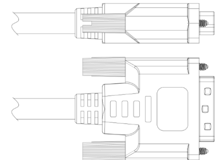
Wire Details(Scale 8:1)
