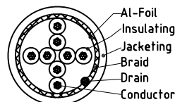
Wire Details
