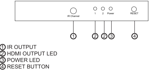
Front Panel
