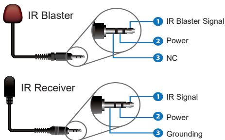
IR Receiver
